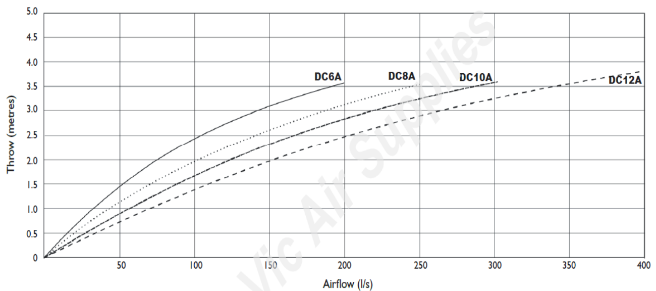
Throw versus Airflow
