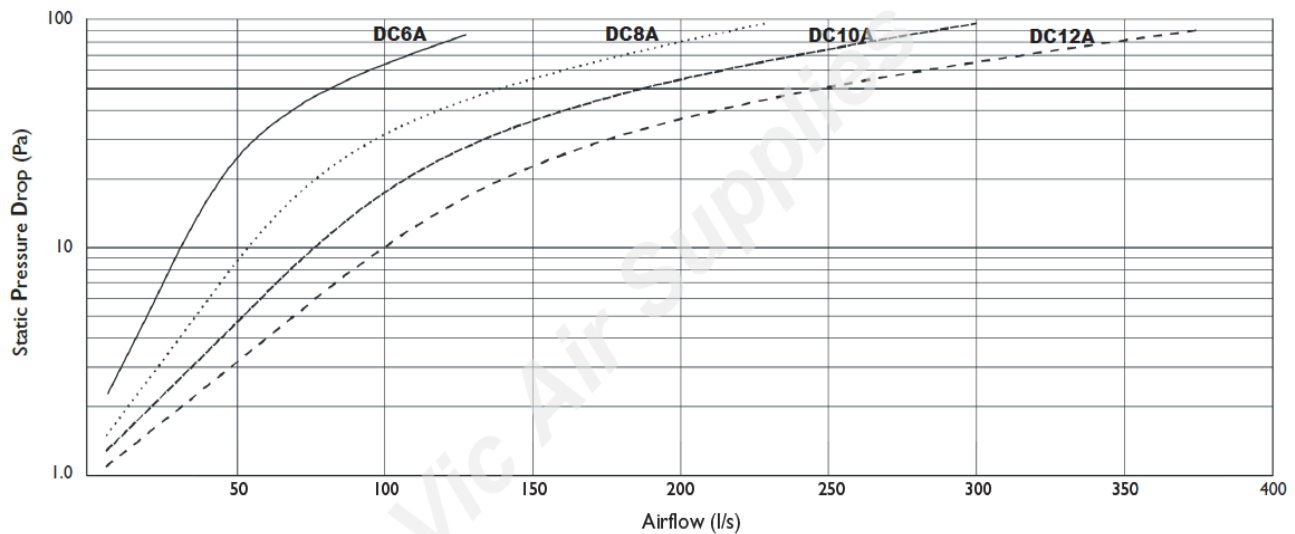
Static Pressure Drop Versus Airflow
